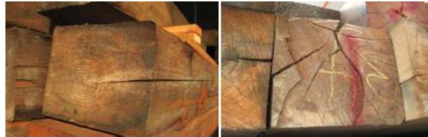
Figure 4. Left: drying cracks in the wood, right: cracks due to overloading
