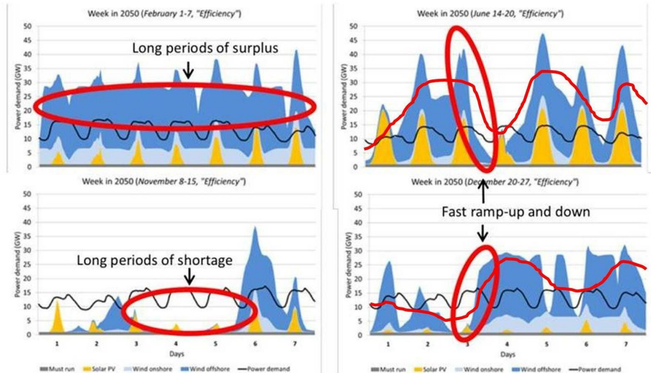
Electricity balance per hour for 2050, selection of weeks
