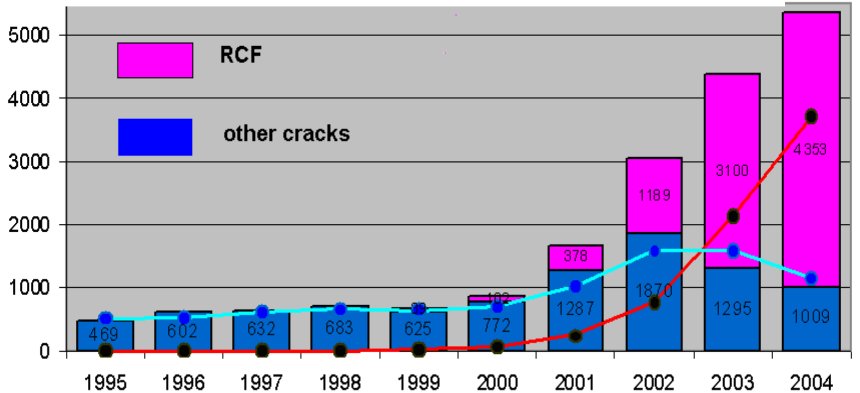
ProRail - ultrasonic defects (pink = due to RCF)
