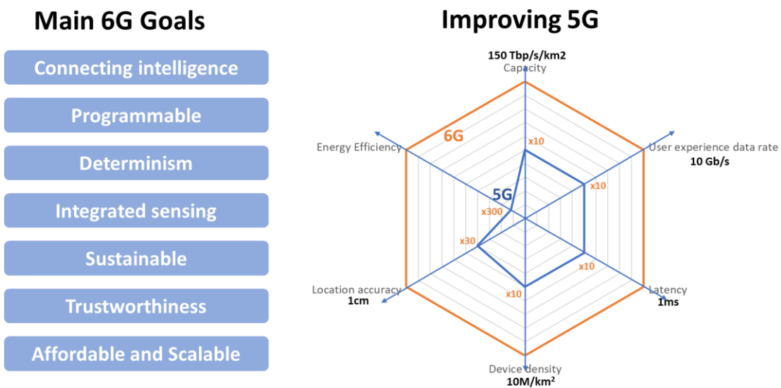
Figure 3.3: 6G goals.
